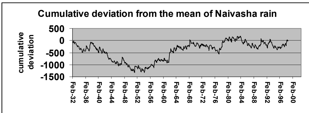
Fig 3: Cumulative deviation from the mean of Naivasha rain.
