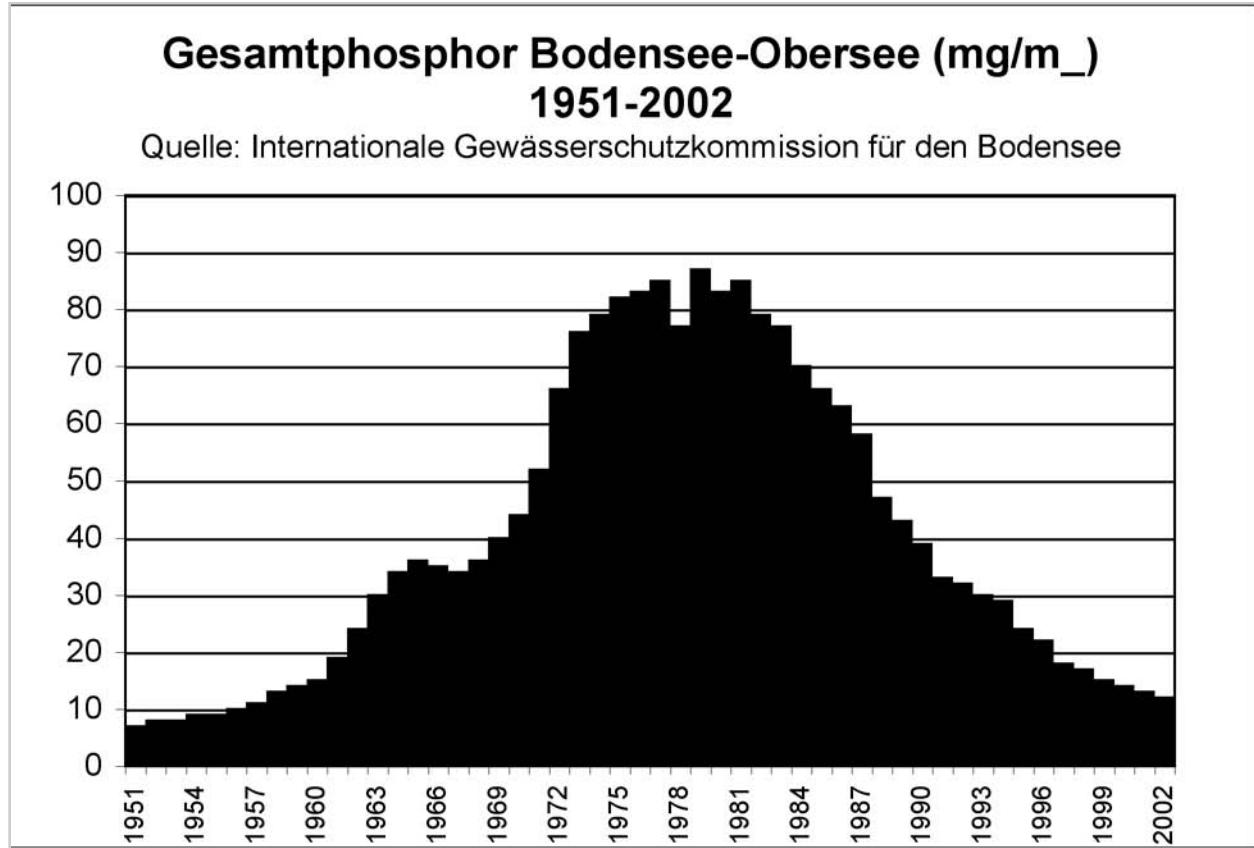
Total Phosphorus, Upper Lake, Lake Constance.
